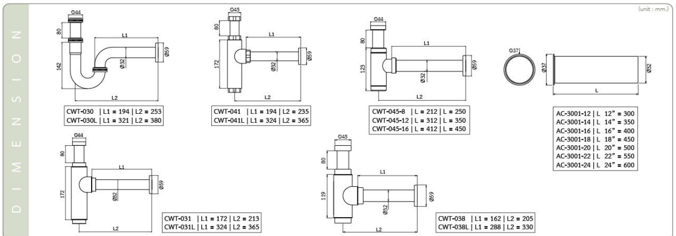
AC-3001-20 • 50 cm. Pipe ( 20" )
