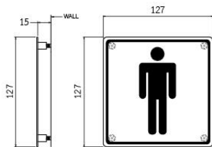
Stainless Steel Sign Plate
