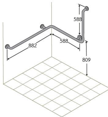
HR-1302-2 Stainless Steel Shower Hand Rail • Made to Order
