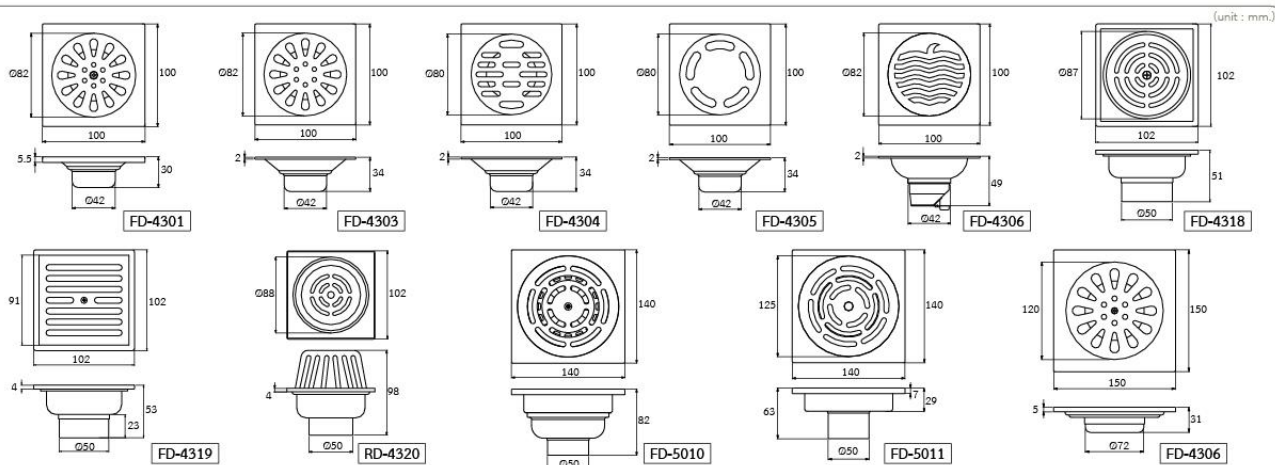
FD-5010 Stainless Steel 5.5" Floor Drain • Drain Rate 22 liters/minute • for 2" - 2.5" PVC Pipe
