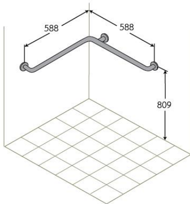
HR-1301-2 Stainless Steel Shower Hand Rail • Made to Order
