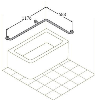
HR-1401-2 Stainless Steel Shower Hand Rail • Made to Order
