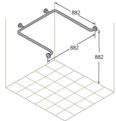
HR-1303-2 Stainless Steel Shower Hand Rail • Made to Order
