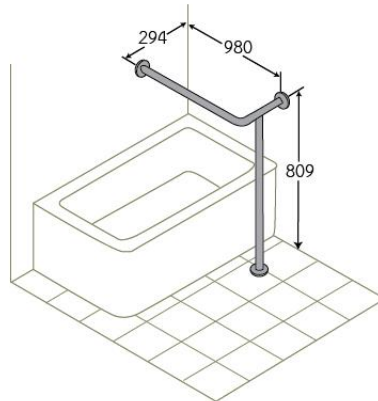
HR-1402-2 Stainless Steel Shower Hand Rail • Made to Order
