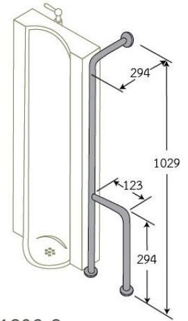
HR-1203-2 Stainless Steel Urinal Hand Rail • Made to Order
