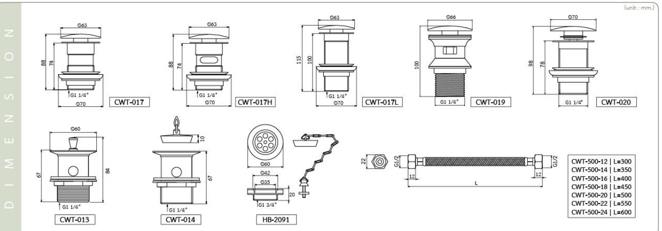
CWT-500-20N • Length 50 cm. (20")
